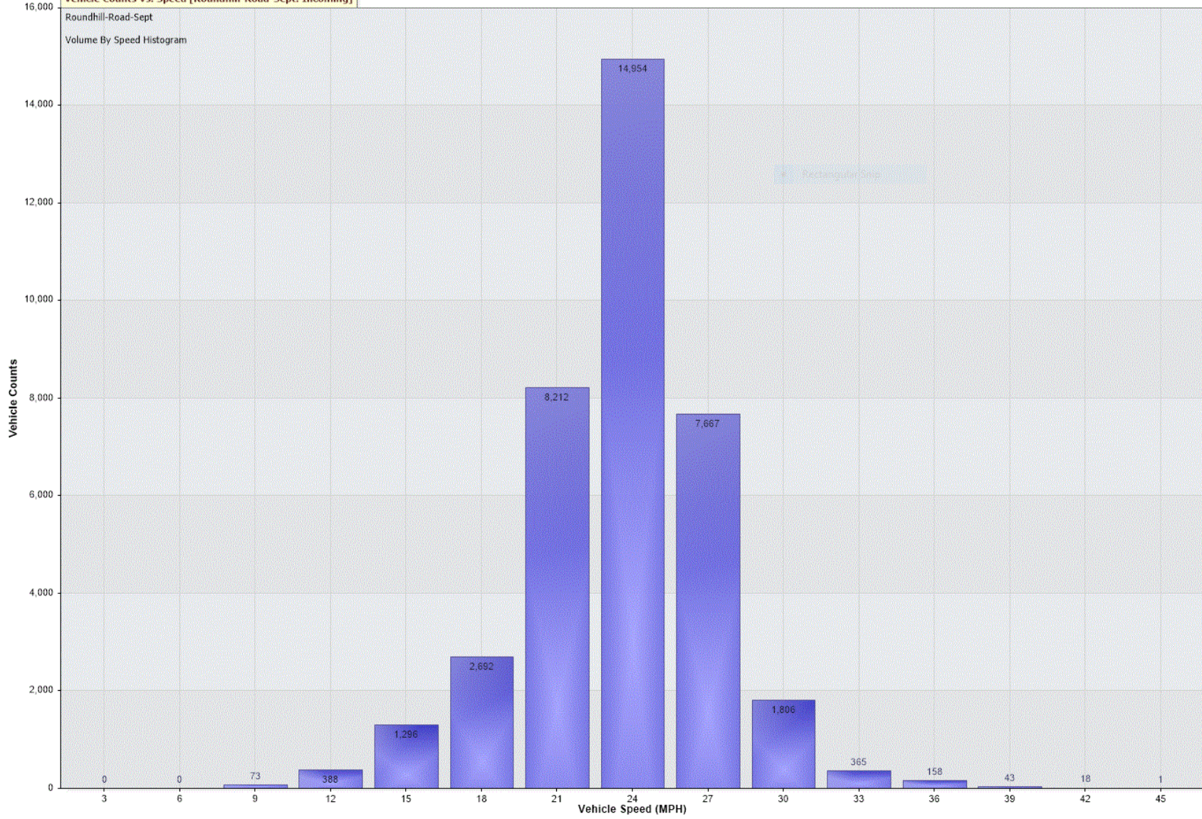
Vehicle Counts Vs. Speed [Roundhill-Road-Sept: Incoming]
