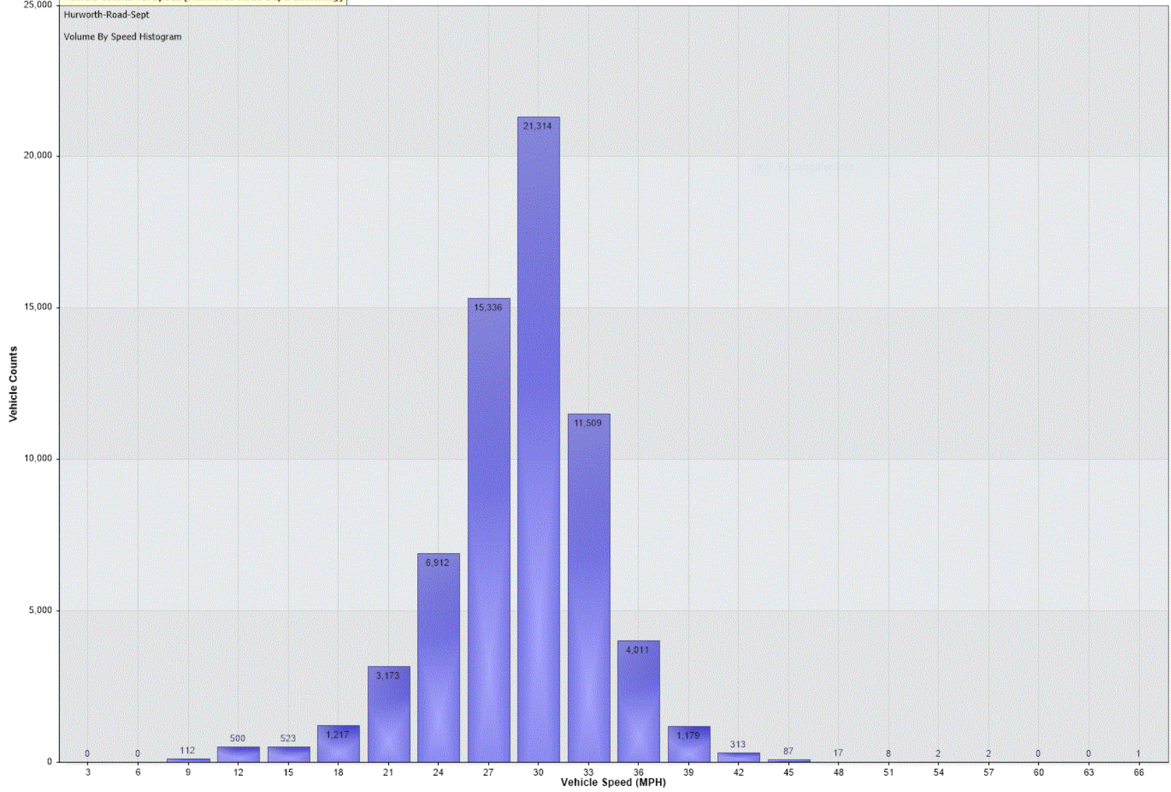
Vehicle Counts Vs. Speed [Hurworth-Road-Sept: Incoming]
