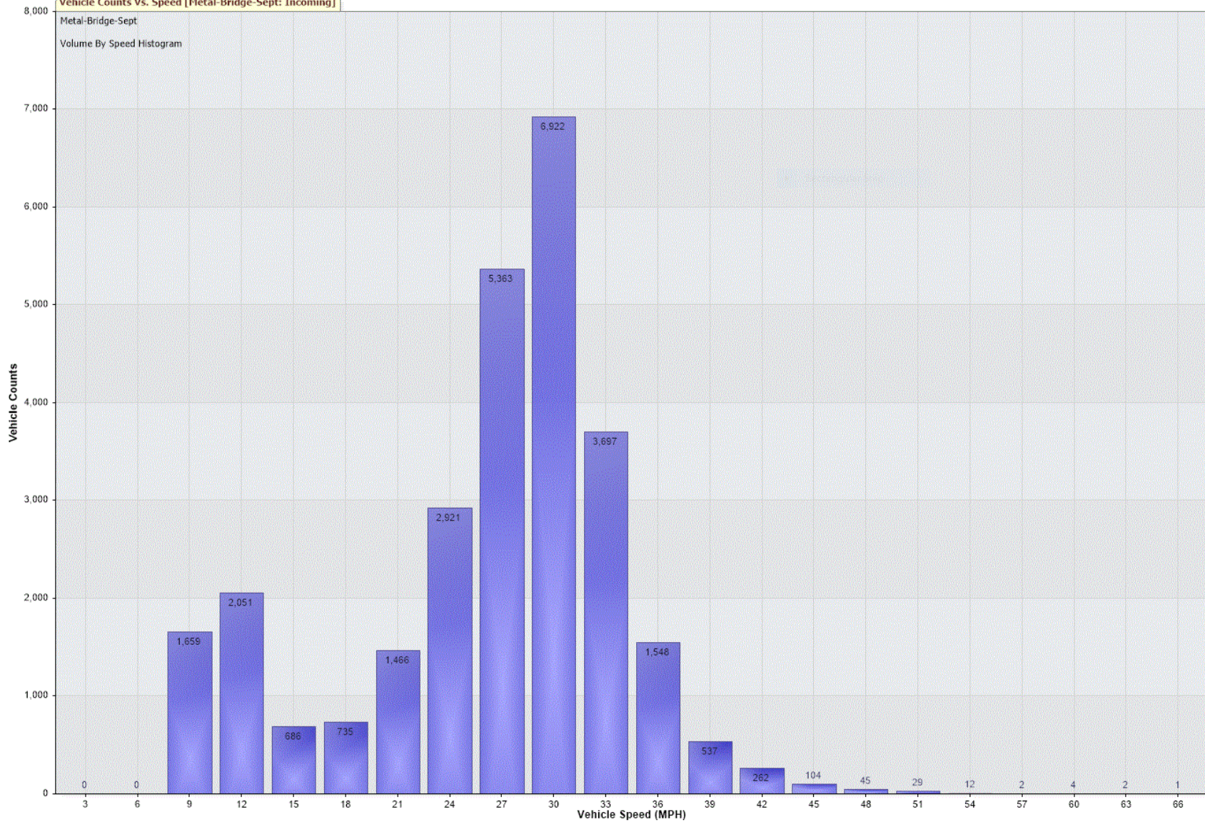
Vehicle Counts Vs. Speed [Metal-Bridge-Sept: Incoming]
