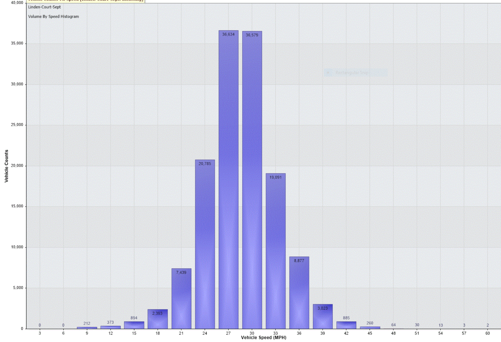
Vehicle Counts Vs. Speed [Linden-Court-Sept: Incoming]
