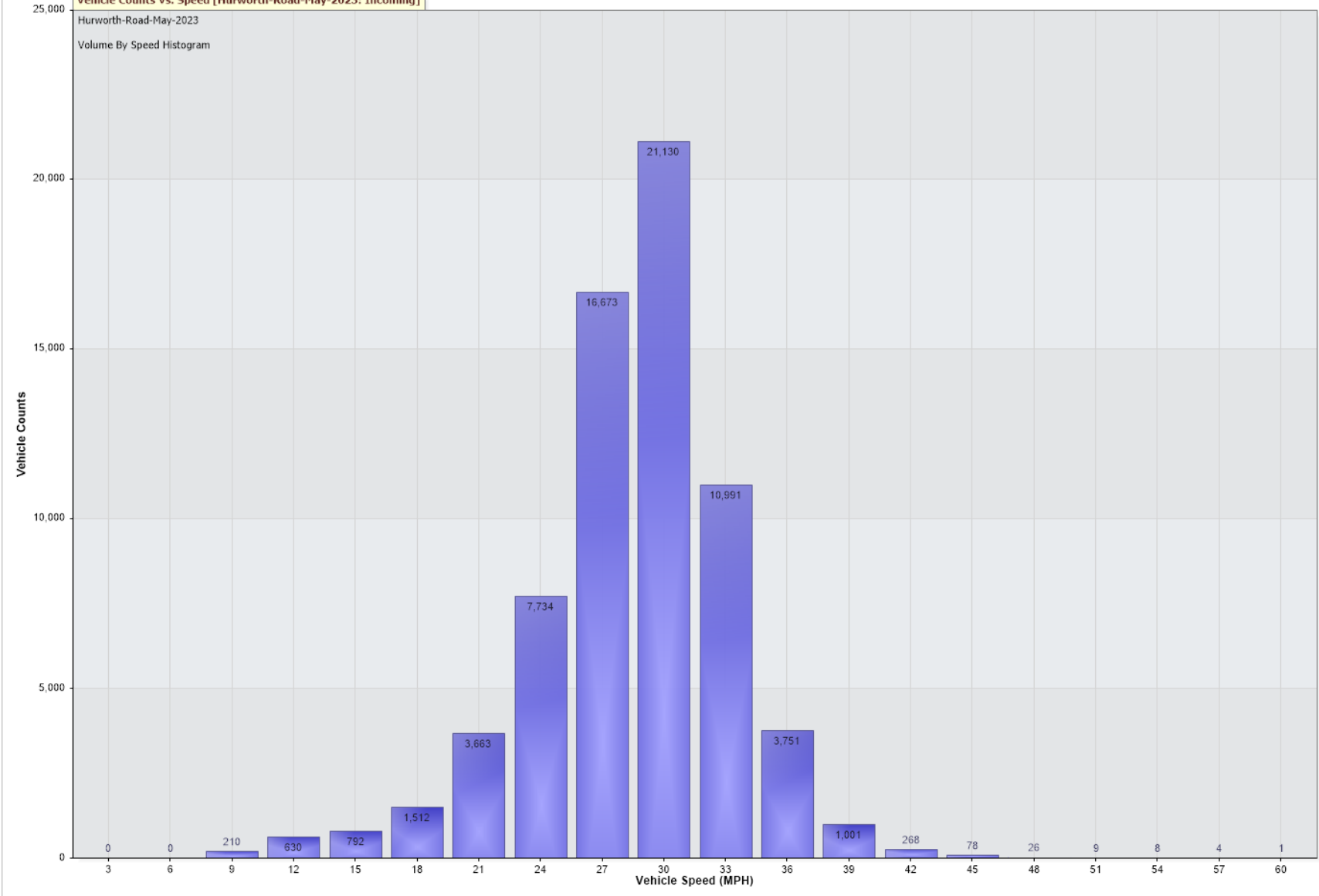
Vehicle Counts Vs. Speed [Hurworth-Road-May-2023: Incoming]
