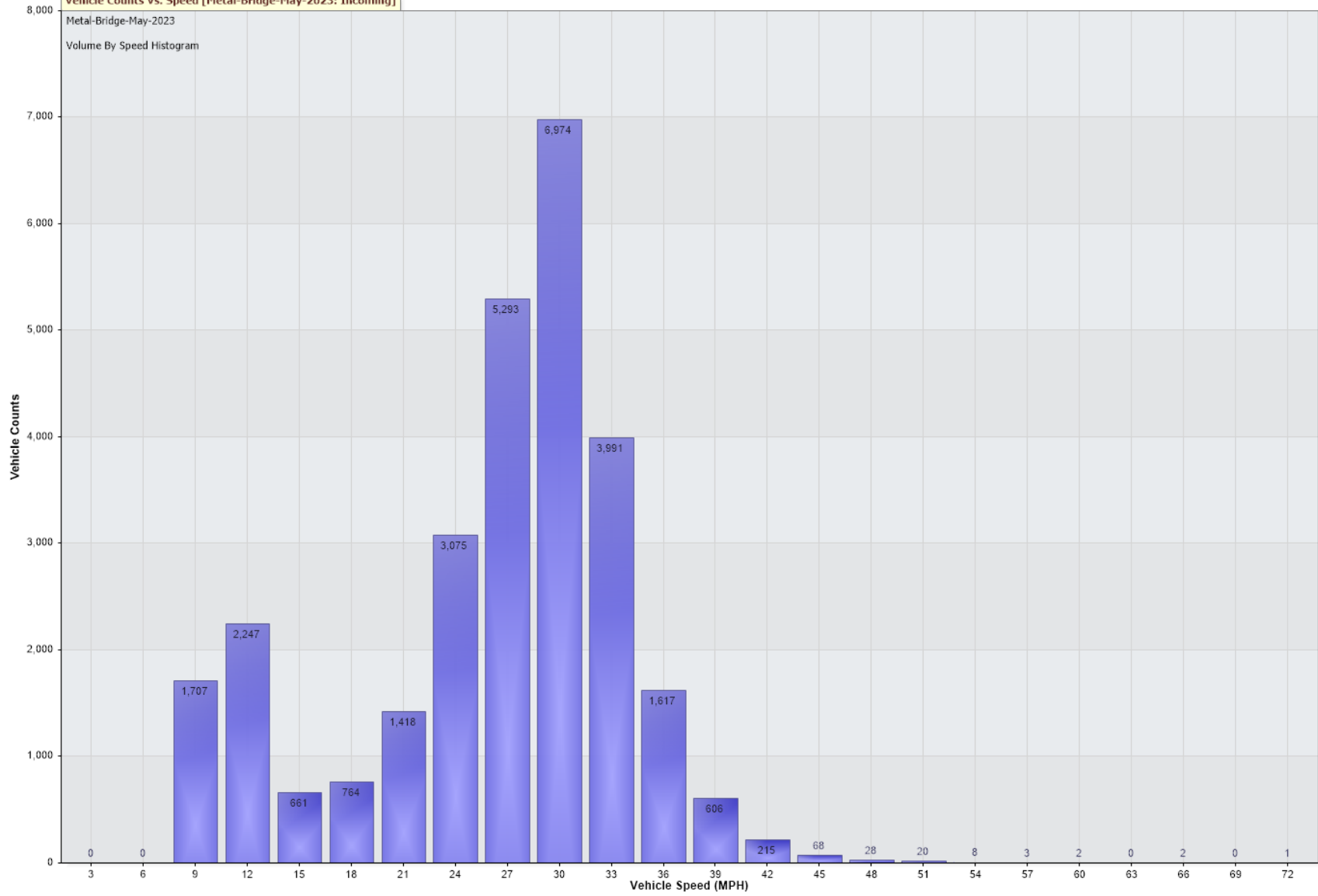
Vehicle Counts Vs. Speed [Metal-Bridge-May-2023: Incoming]
