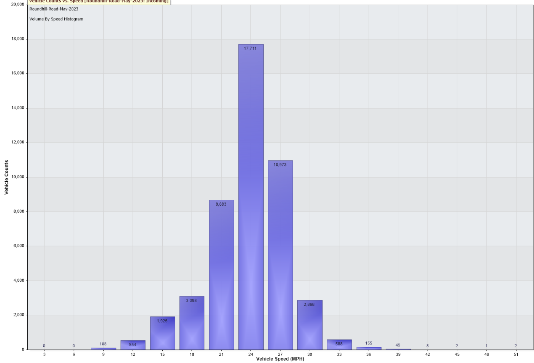
Vehicle Counts Vs. Speed [Roundhill-Road-May-2023: Incoming]
